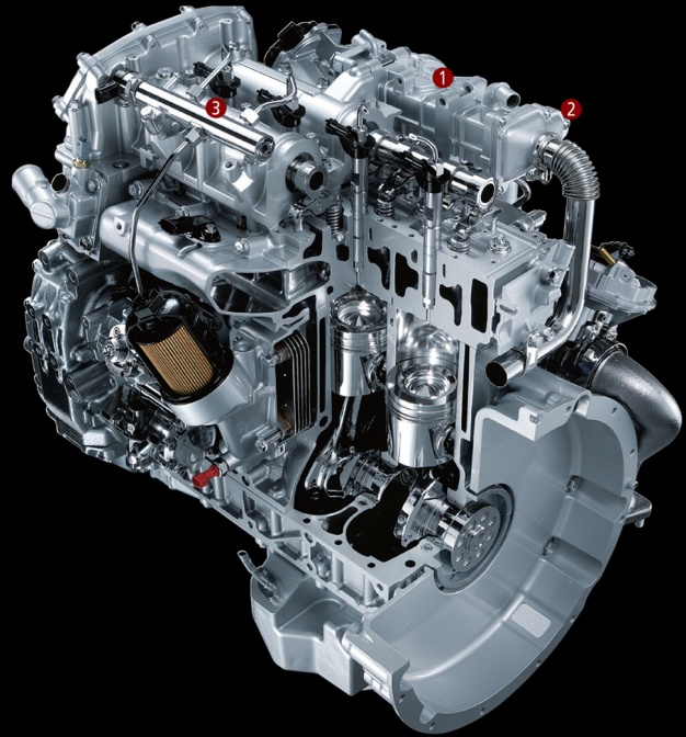
1 HIGH PRECISION COOLED EGR SYSTEM *EGR: Exhaust Gas Recirculation
